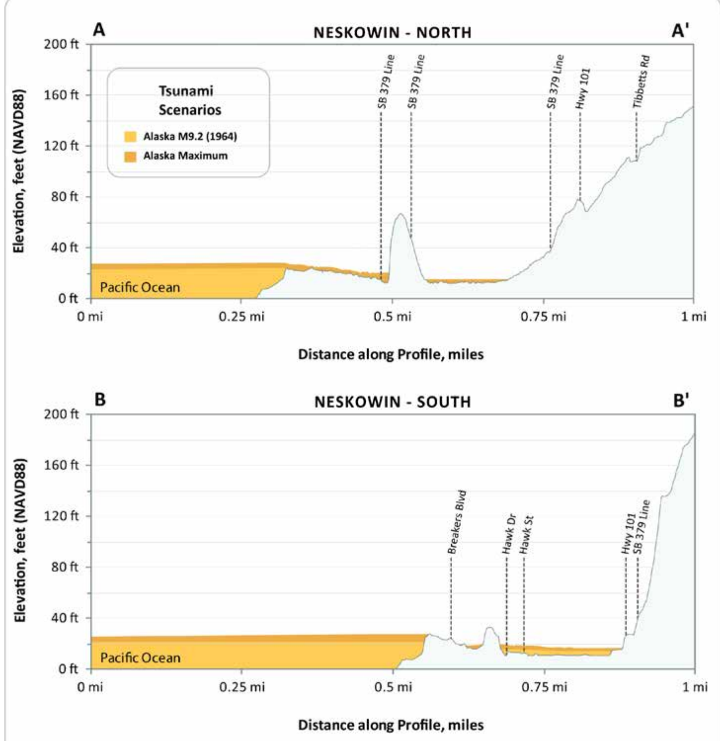
Figure 5. These profiles depict the expected maximum tsunami wave elevation for the two Alaska tsunami scenarios along lines A-A' and B-B'. The tsunami scenarios are modeled to occur at a (no flow) tide and equal to the Mean Higher High Water (MHHW) high tide.
