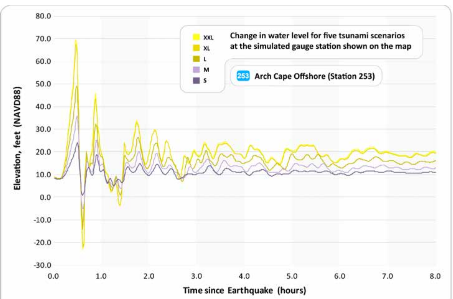
Figure 5: This chart depicts the tsunami waves as they arrive at the selected reference point (simulated gauge station). It shows the change in wave heights for all the tsunami scenarios over an 8-hour period. The starting wave elevation (0.0 hour) takes into account the local land subsidence or uplift caused by the earthquake. Wave heights vary through time, and the first wave will not necessarily be the largest as waves interfere and reflect off local topography and bathymetry. Any absence of data indicates periods for which tsunami inundation has not yet reached or has receded from the station location and dry land is exposed.
