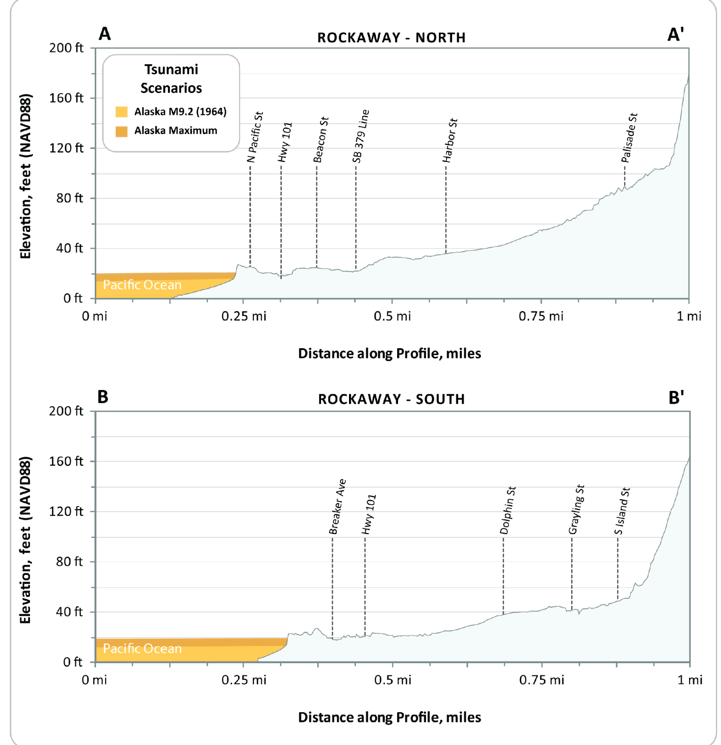
Figure 5: These profiles depict the expected maximum tsunami wave elevation for the two Alaska tsunami scenarios along profiles A-A' and B-B'. The tsunami scenarios are modeled to occur at a static (no flow) tide and equal to the Mean Higher High Water (MHHW) high tide.
