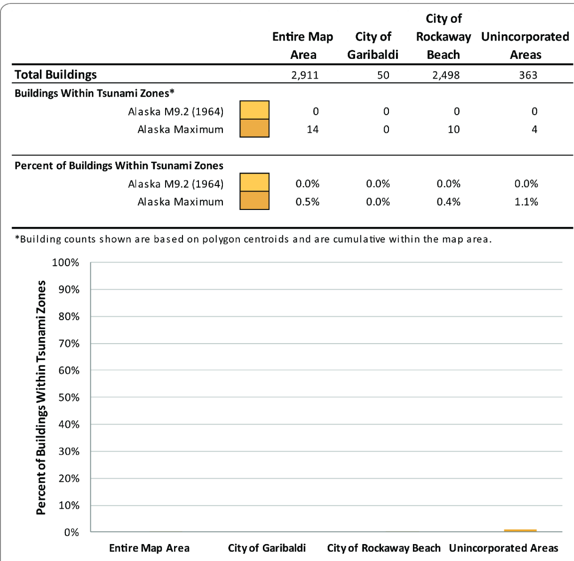
Figure 3: The table and chart show the number of buildings inundated for the Alaska M9.2 (1964) and the Alaska Maximum tsunami scenarios for the cities and unincorporated portions of the map.
