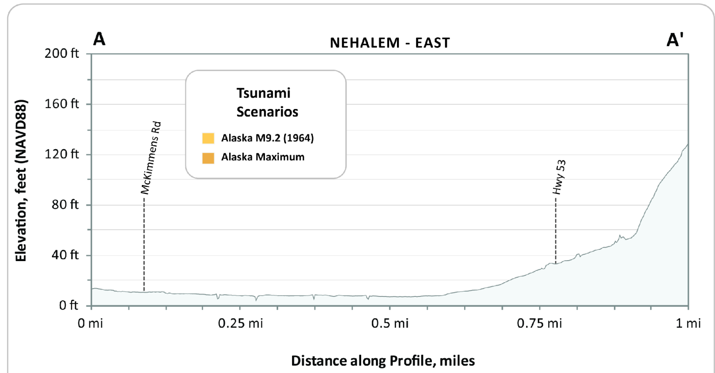
Figure 5: This profile depicts the expected maximum tsunami wave elevation for the two Alaska tsunami scenarios along line A-A'. The tsunami scenarios are modeled as water at static (no flow) tide and equal to the Mean Higher High Water (MHHW) tide.
