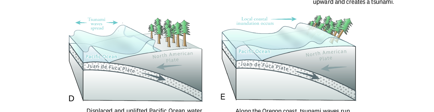
Figure 3: Along the Oregon coast, tsunami waves run up onto the land for several hours. Displaced and uplifted Pacific Ocean water rushes in all directions.
