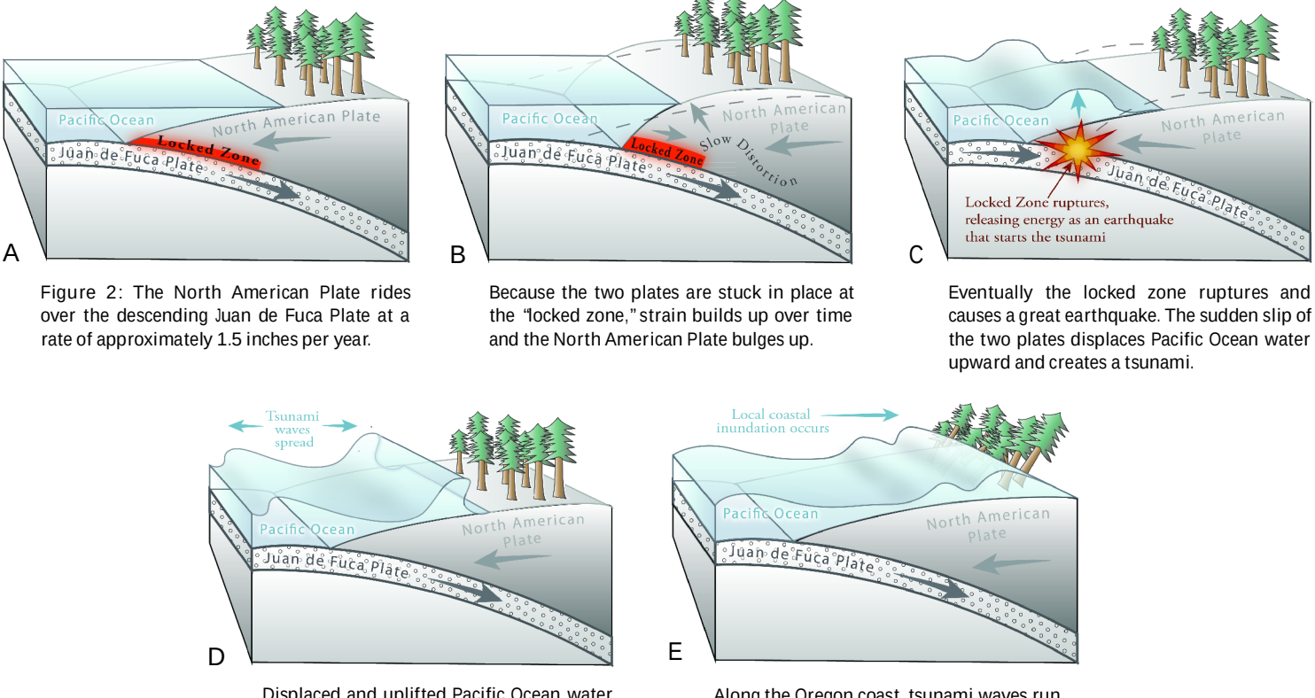
Figure 3: Along the Oregon coast, tsunami waves run up onto the land for several hours. Displaced and uplifted Pacific Ocean water rushes in all directions.
