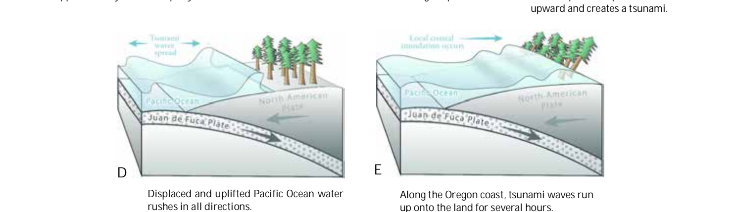
Figure 2 (continued): Displaced and uplifted Pacific Ocean water rushes in all directions.
