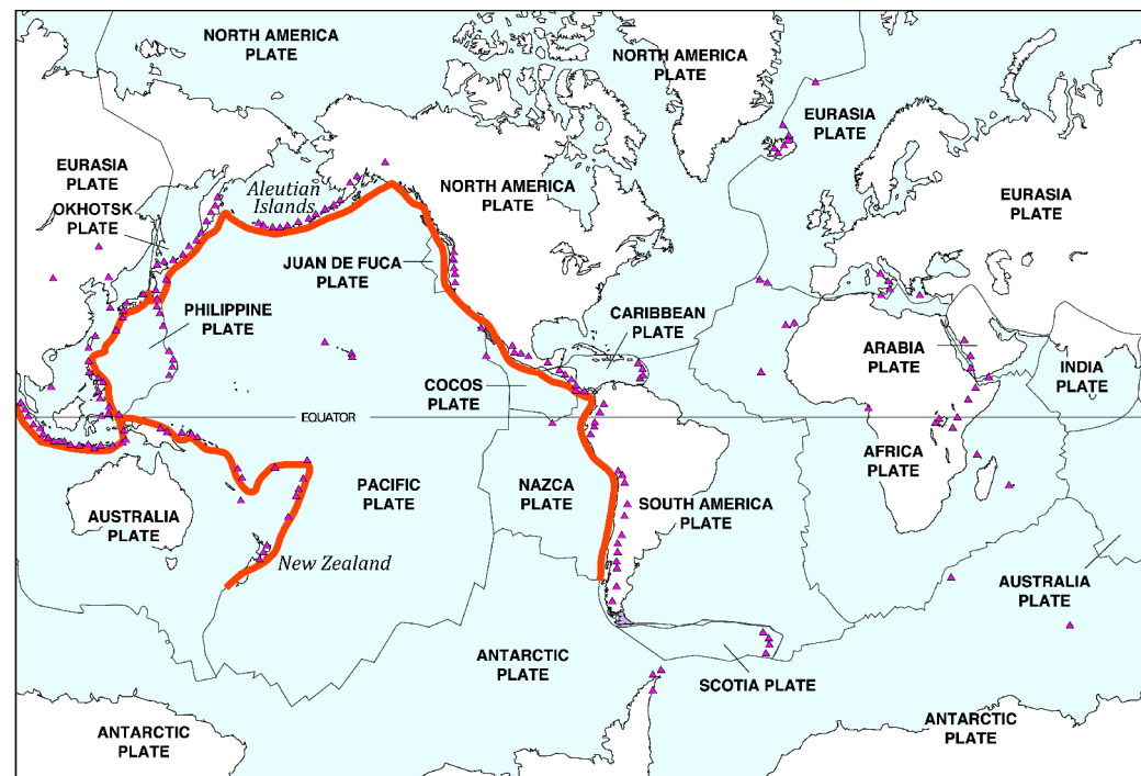
Figure 1. The "Ring of Fire" is a zone of active earthquakes and volcanoes that encircles much of the Pacific Ocean, including the Oregon coast. Volcanoes and earthquakes on this ring are caused by the movements of tectonic plates. One type of movement is called subduction - when thin, oceanic plates sink beneath thicker, lighter plates that make up continental plates. Earthquakes that occur as a result of subduction can trigger tsunamis.
