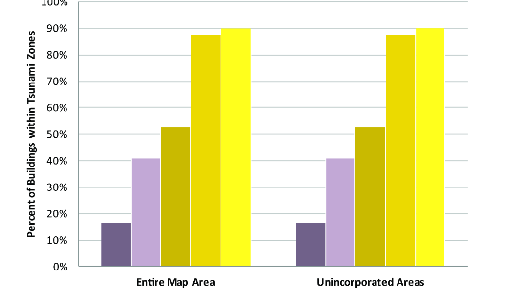
Figure 4: The table and chart show the number of buildings inundated by each tsunami T-shirt scenario for cities and unincorporated portions of the map.
