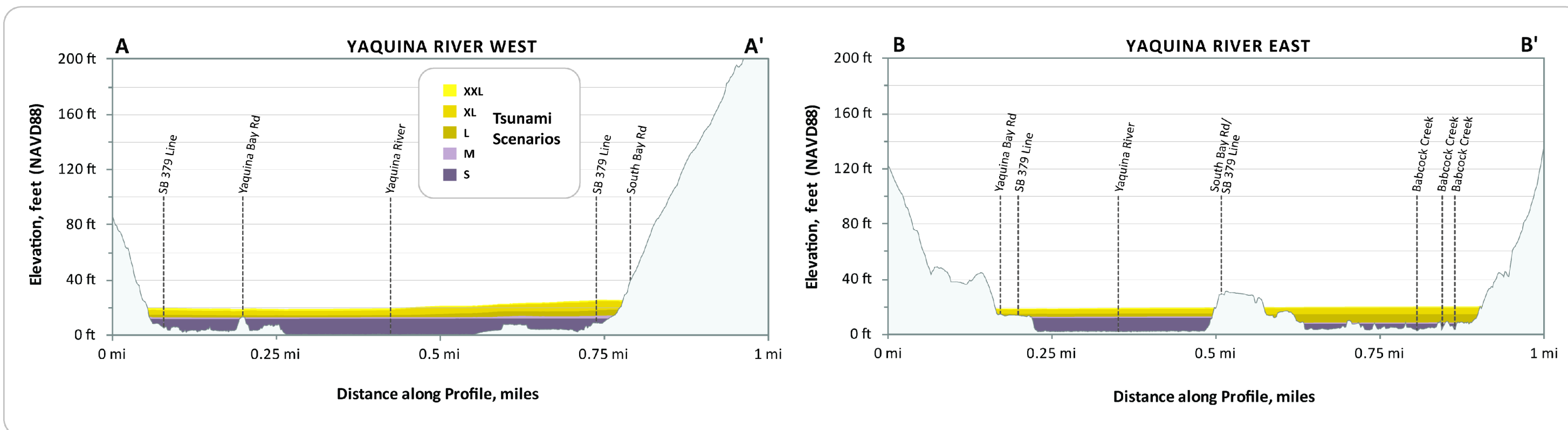
Figure 6: These profiles depict the expected maximum tsunami wave elevation for the five 'T-shirt' scenarios 'along lines A-A' and B-B'. The tsunami scenarios are modeled to occur at high tide and to account for local subsidence or uplift of the ground surface.
