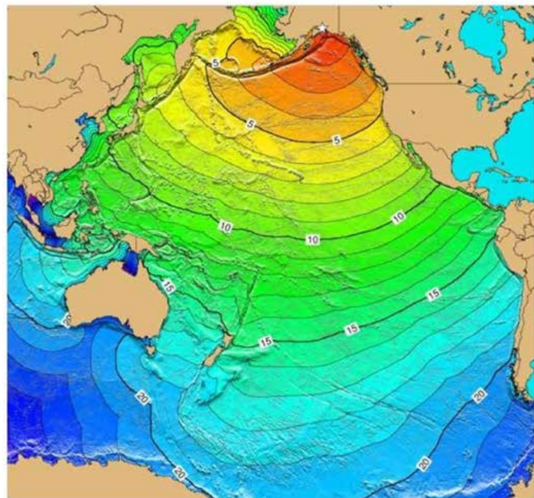
Figure 2: This image depicts the initial tsunami arrival times in hours around the Pacific Rim from the 1964 Prince William Sound earthquake. This magnitude 9.2 earthquake and resulting tsunami caused 125 deaths and $311 million in property loss, 884 million and 109 deaths in Alaska (NOGIC/WOC). The tsunami devastated many towns along the Gulf of Alaska, left serious damage in British Columbia, Hawaii, and along the west coast of the United States, and was recorded on tide gauges in Cuba and Puerto Rico.
