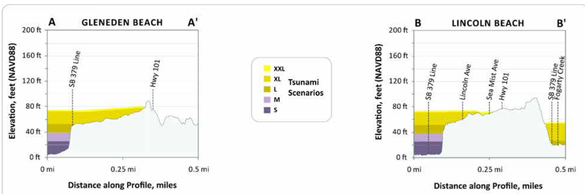
Figure 6: These profiles depict the expected maximum tsunami wave elevation for the five "T-shirt" scenarios along lines A-A' and B-B'. The tsunami scenarios are modeled to occur at high tide and to account for local subsidence or uplift of the ground surface.
