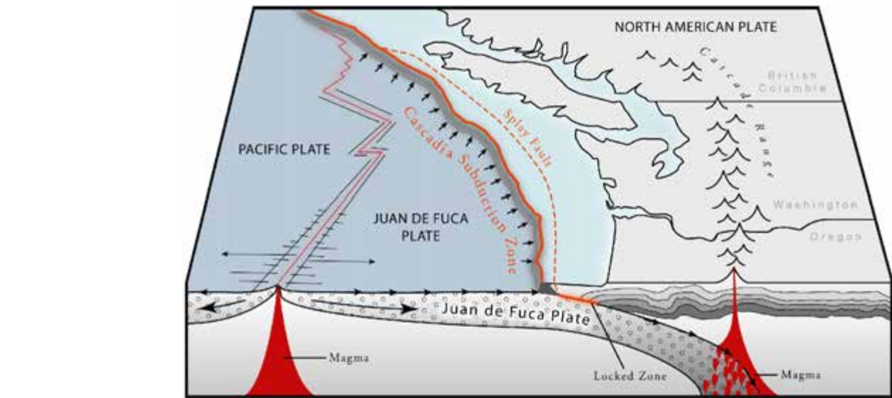
Figure 1: This block diagram depicts the tectonic setting of the region. See Figure 2 for the sequence of events that occur during Cascadia Subduction Zone megathrust earthquake and tsunami.
