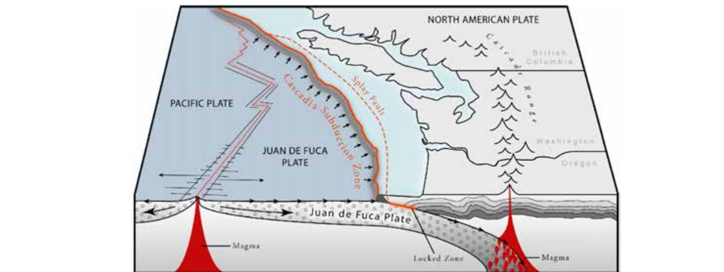
Figure 1: This block diagram depicts the tectonic setting of the region. See Figure 2 for the sequence of events that occur during Cascadia Subduction Zone megathrust earthquake and tsunami.
