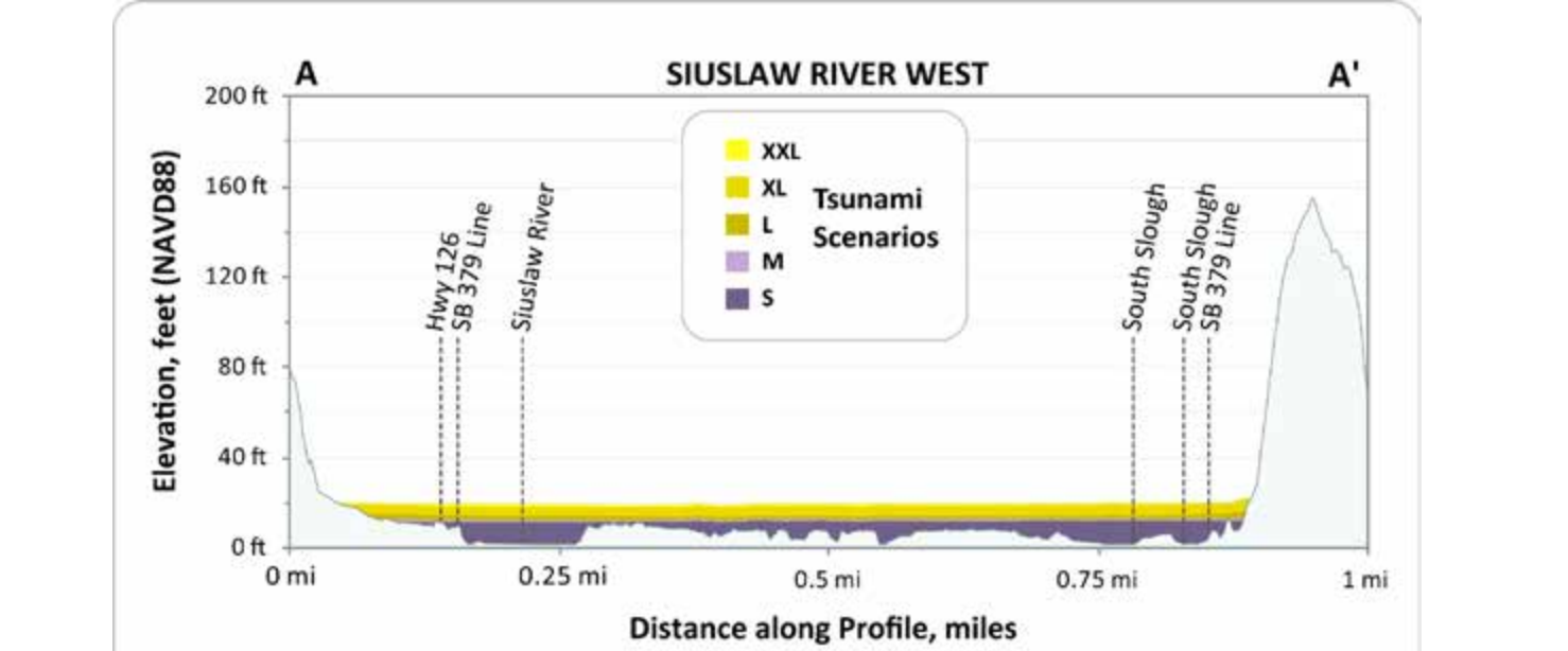
Figure 7: Three profiles depict the expected maximum tsunami wave elevation for the five 'T-shirt size' scenarios along lines A-A' and B-B'. The tsunami scenarios are modeled to occur at high tide and account for local subsidence or uplift of the ground surface.
