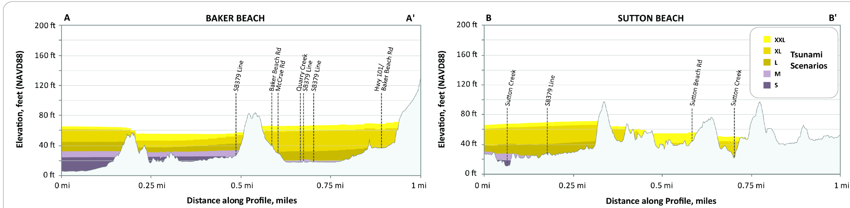
Figure 6: These profiles depict the expected maximum tsunami wave elevation for the five 'T-shirt' scenarios along lines A-A' and B-B'. The tsunami scenarios are modeled to occur at high tide and to account for local subsidence or uplift of the ground surface.
