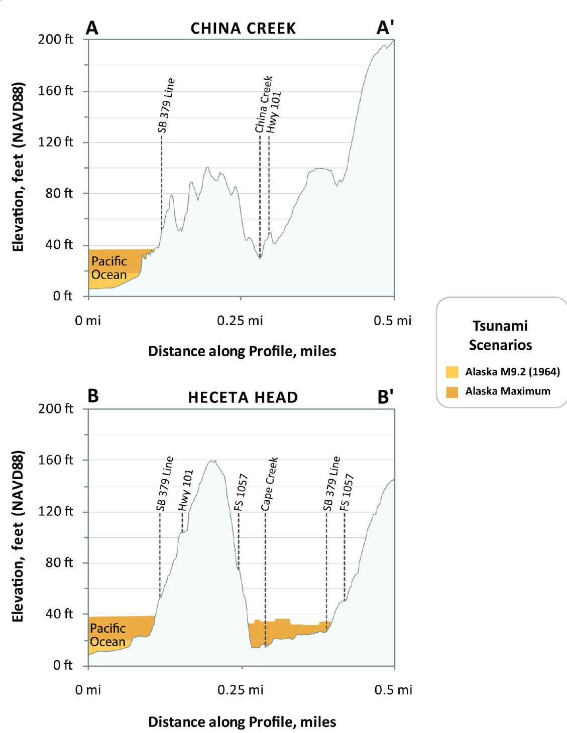
Figure 5: These profile depict the expected maximum tsunami wave elevation for the two Alaska tsunami scenarios along lines A-A' and B-B'. The tsunami scenarios are modeled to occur as a static (no flow) tide and equal to the Mean Higher High Water (MHHW) high tide.
