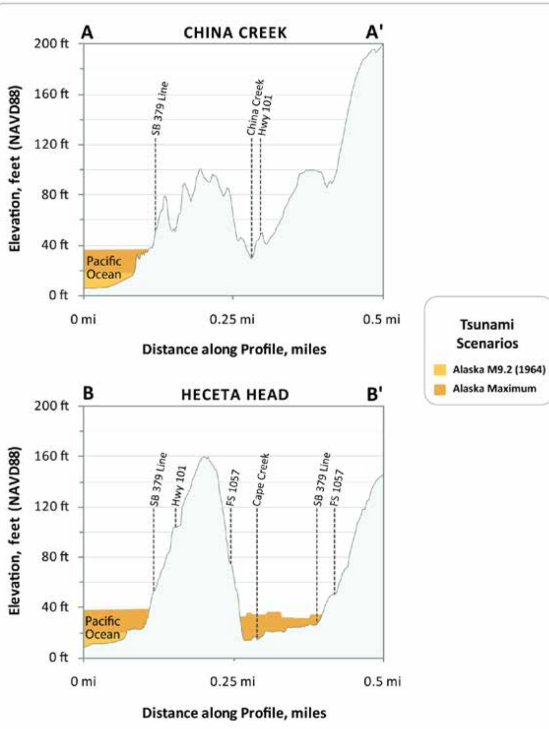
Figure 5: These profile depict the expected maximum tsunami wave elevation for the two Alaska tsunami scenarios along lines A-A' and B-B'. The tsunami scenarios are modeled to occur as a static (no flow) tide and equal to the Mean Higher High Water (MHHW) high tide.
