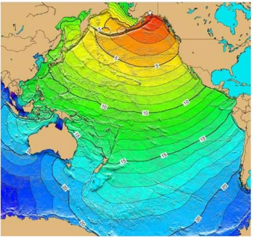
Figure 2: This image depicts the tsunami travel time in hours, around the Pacific Rim from the 1964 M9.2 Prince William Sound earthquake. This magnitude 9.2 earthquake and resulting tsunami caused 125 deaths and $3.1 billion in property loss, 584 million and 100 deaths in Alaska (NODC/WDC). The tsunami devastated many towns along the Gulf of Alaska, left serious damage in British Columbia, Hawaii, and along the west coast of the United States, and was recorded on tide gauges in Cuba and Puerto Rico.
