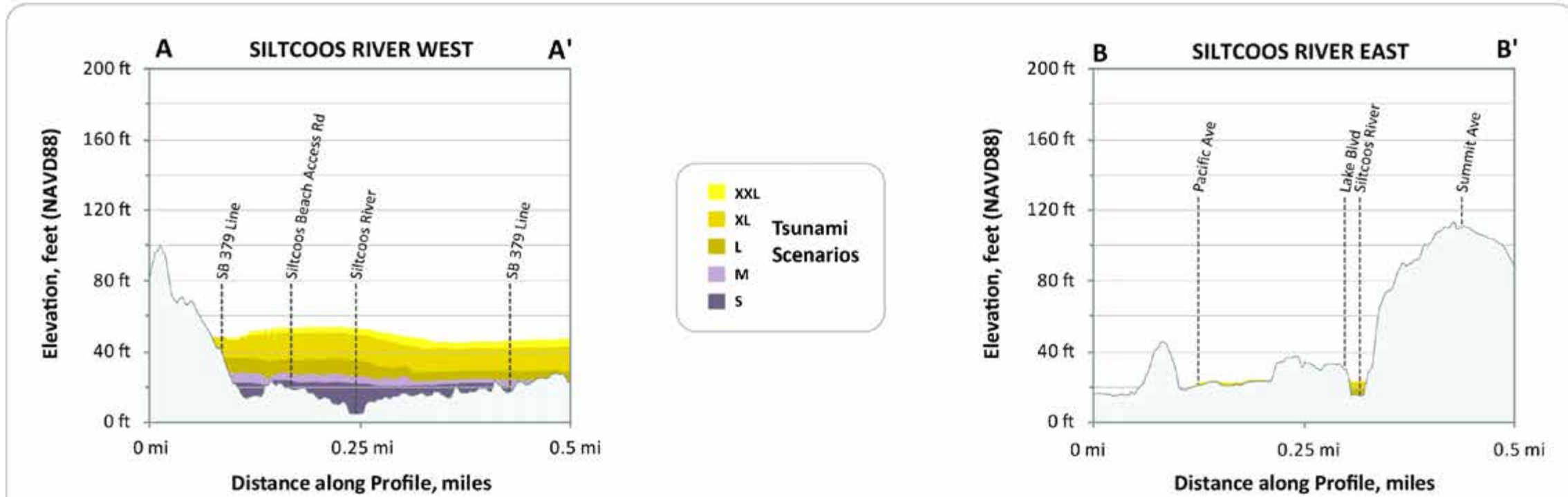
Figure 6: These profiles depict the expected maximum tsunami wave elevation for the five "Tsunami T-shirt scenarios" along lines A-A' and B-B'. The tsunami scenarios are modeled to occur at high tide and to account for local subsidence or uplift of the ground surface.
