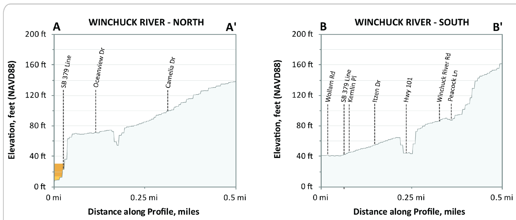
Figure 5: These profiles depict the expected maximum tsunami wave elevation for the two Alaska tsunami scenarios along lines A-A' and B-B'. The tsunami scenarios are modeled to occur at static (no flow) tide and equal to the Mean Higher High Water (MHHW) high tide.
