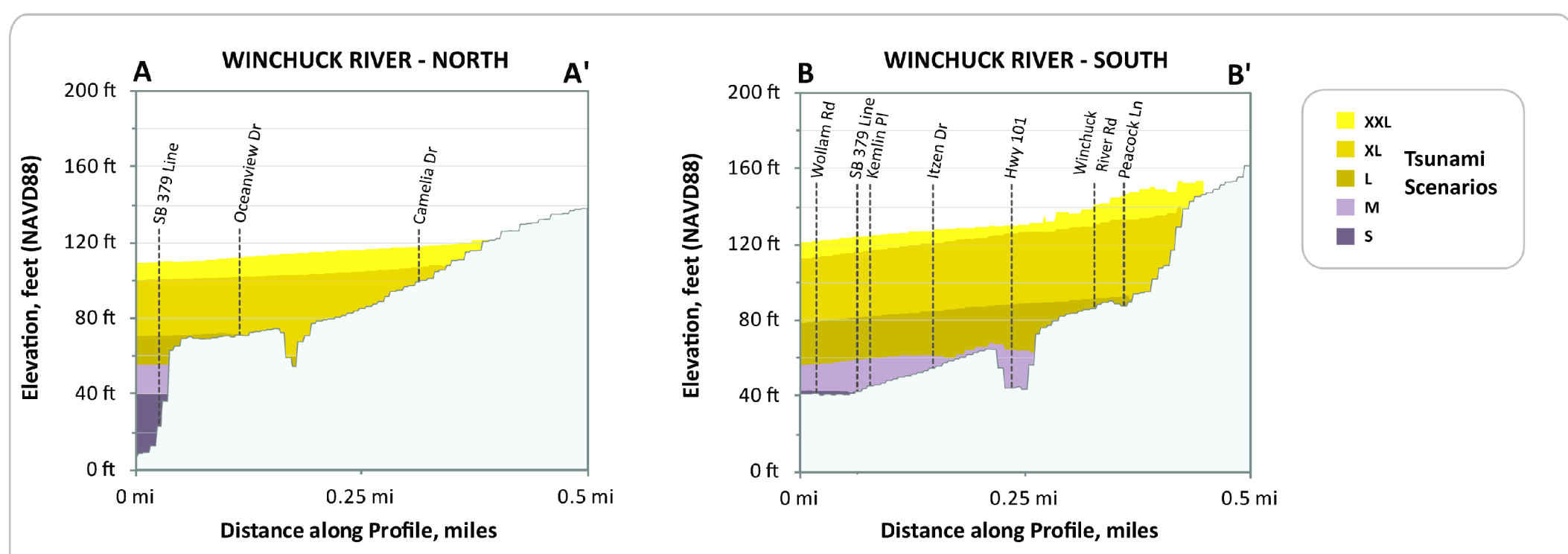
Figure 6: These profiles depict the expected maximum tsunami wave elevation for the five "T-shirt size" scenarios along lines A-A' and B-B'. The tsunami scenarios are modeled to occur at high tide and to account for local subsidence or uplift of the ground surface.
