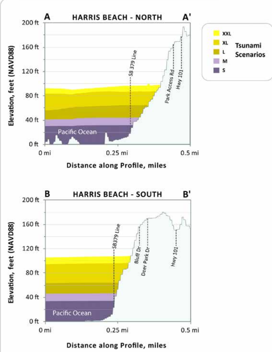
Figure 6. These graphs depict the expected maximum tsunami wave elevation for the five "T-shirt" scenarios along lines A-A' and B-B'. The tsunami scenarios are modeled to occur at high tide and to account for local subsidence or uplift of the ground surface.
