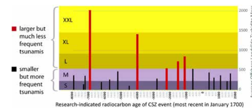
Figure 3. This chart depicts the timing, frequency, and magnitude of the last 19 great Cascadia Subduction Zone events over the past 10,000 years. The most recent event occurred in January 26, 1700. The 1700 event is considered to be a "medium sized" event. The data used to create this chart came from research that examined the many "summer" tsunamis, known as "tsunamis" that are triggered only by these great earthquakes (Witter and others, 2011). The lower correlation is "the larger the tsunamis, the bigger the earthquakes."
