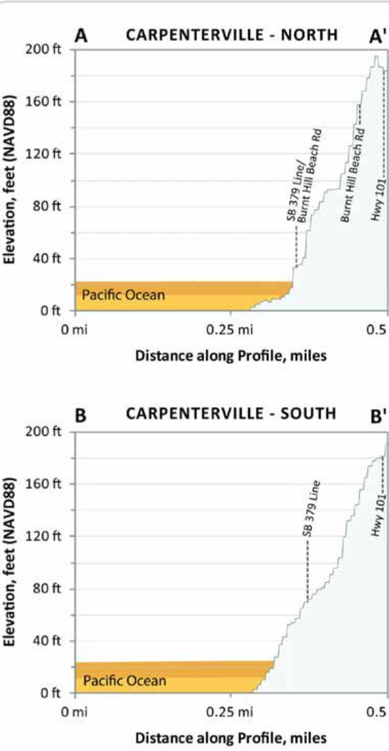
Figure 5: These profile plots depict the expected maximum tsunami wave elevation for the two Alaska tsunami scenarios along lines A-A' and B-B'. The tsunami scenarios are modeled to occur at a static (no flow) tide and equal to the Mean Higher High Water (MHHW) high tide.
