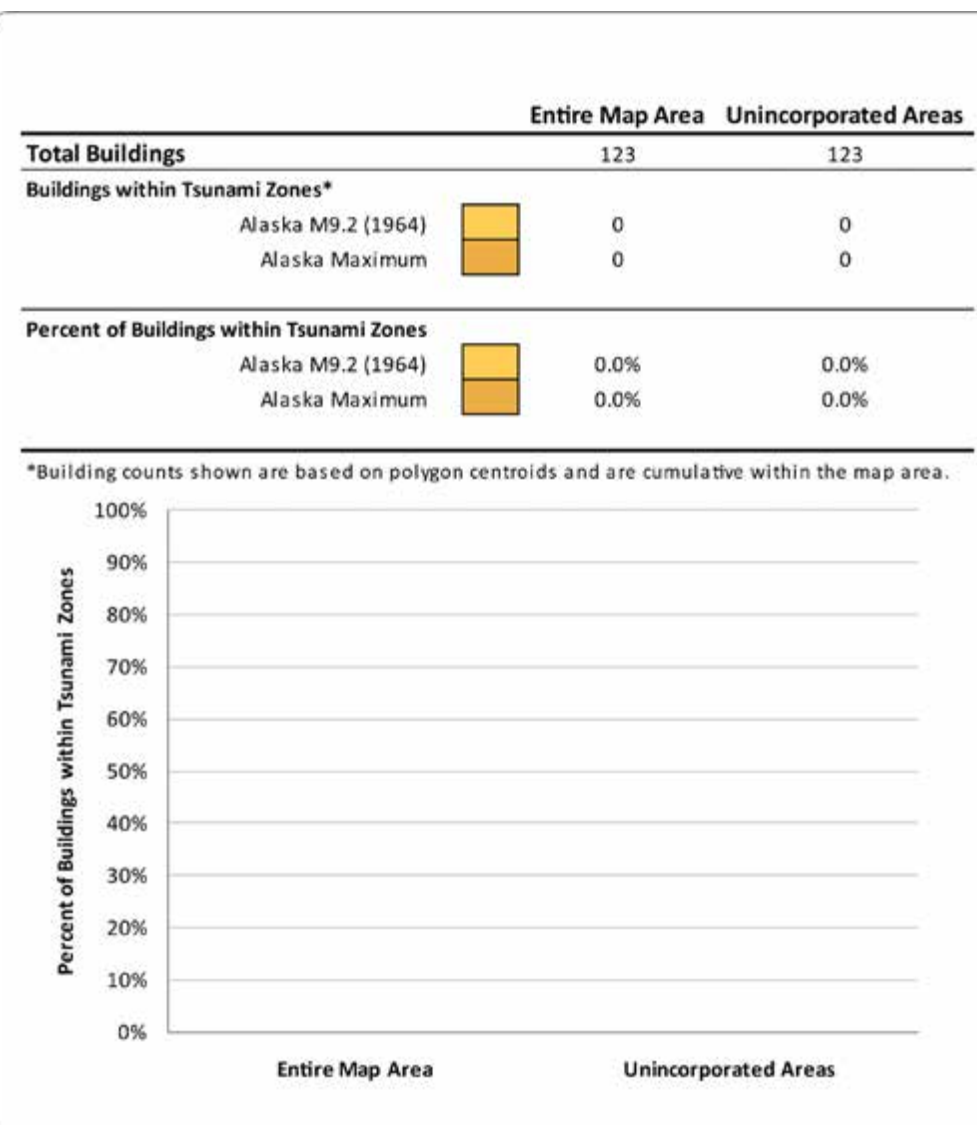
Figure 3: The table and chart show the number of buildings inundated for the Alaska M9.2 (1964) and the Alaska Maximum tsunami scenarios for cities and unincorporated portions of the map.
