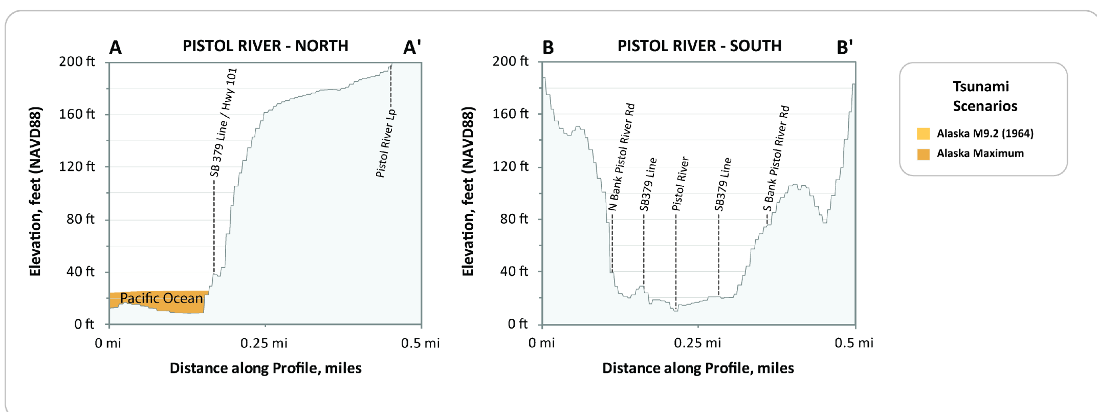
Figure 5: These profiles depict the expected maximum tsunami wave elevation for the two Alaska tsunami scenarios along lines A-A' and B-B'. The tsunami scenarios are modeled to static (no flow) tide and equal to the Mean Higher High Water (MHHW) high tide.
