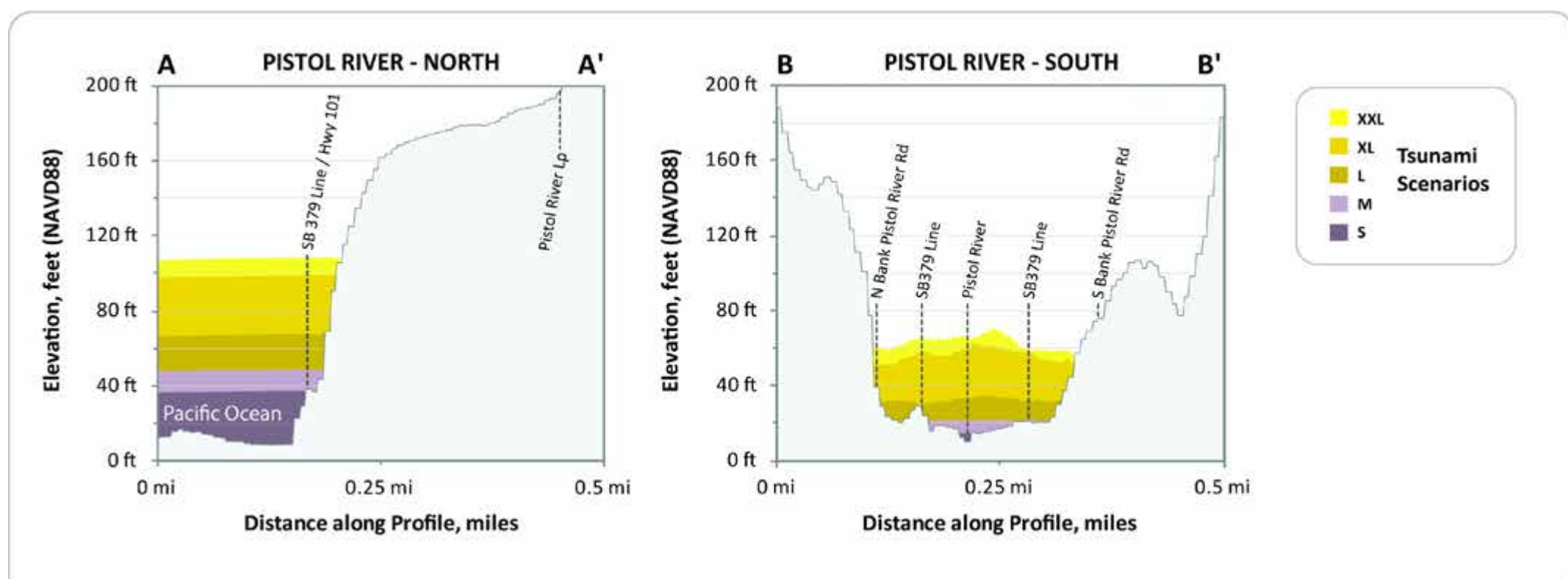
Figure 6: These profiles depict the expected maximum tsunami wave elevation for the five "T-shirt" scenarios along lines A-A' and B-B'. The tsunami scenarios are modeled to occur at high tide and to account for local subsidence or uplift of the ground surface.
