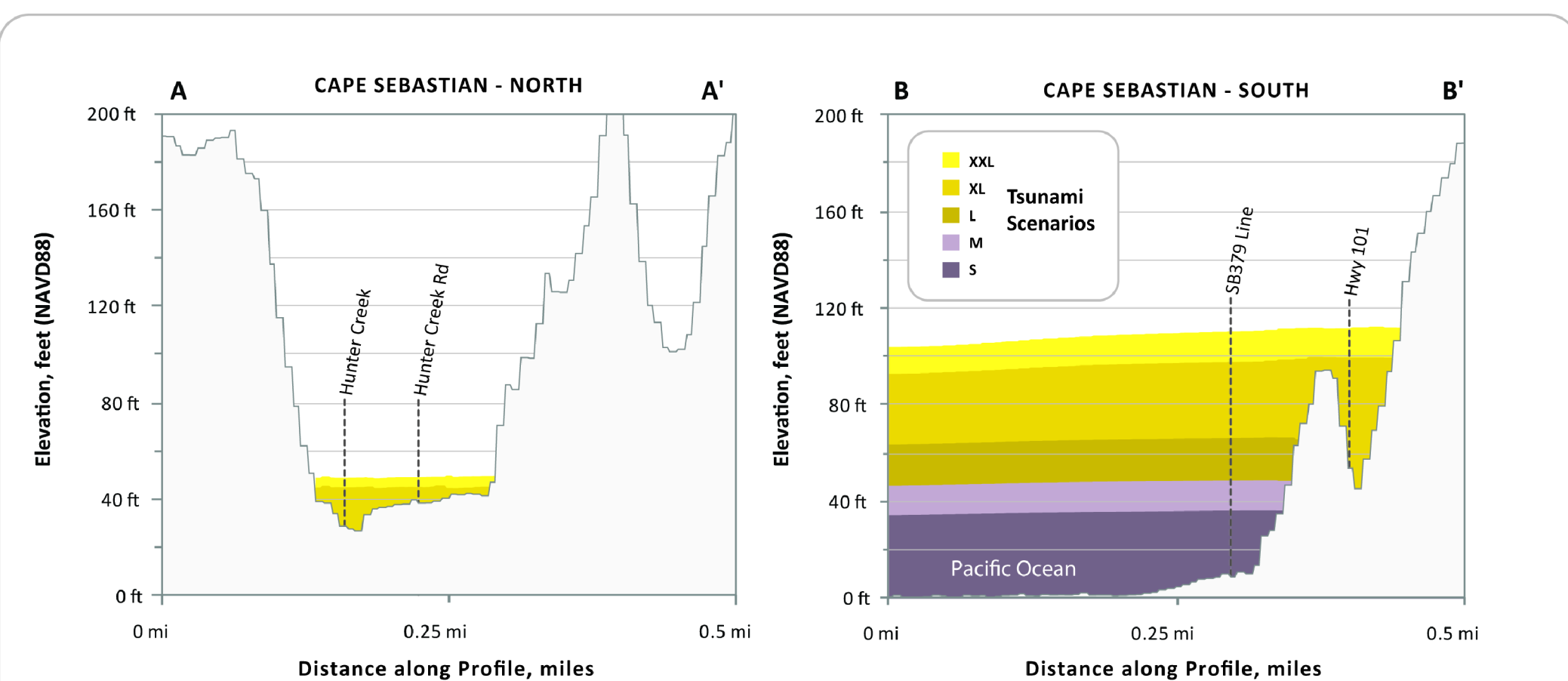
Figure 6: These profiles depict the expected maximum tsunami wave elevation for the five "Tsunami T-shirt scenarios" along lines A-A' and B-B'. The tsunami scenarios are modeled to occur at high tide and to account for local subsidence or uplift of the ground surface.
