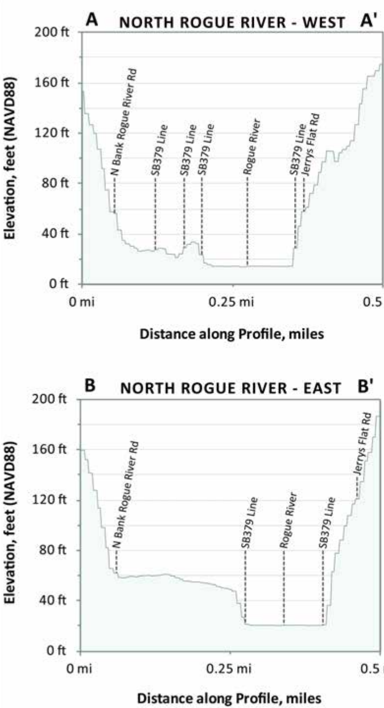
Figure 5: These profiles depict the expected maximum tsunami wave elevation for the two Alaska tsunami scenarios along lines A-A' and B-B'. The tsunami scenarios are modeled to occur at a static (no flow) tide and equal to the Mean Higher High Water (MHHW) high tide.
