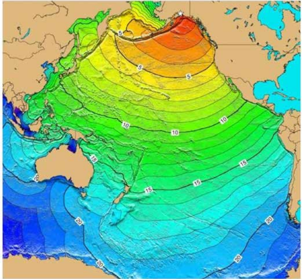
Figure 2: This image depicts the actual initial tsunami arrival times, in hours, around the Pacific Rim from the 1964 Prince William Sound earthquake. The magnitude 9.2 earthquake and resulting tsunami caused 125 deaths and $2.1 million in property loss. $4 million and 100 deaths in Alaska (NOGS 1965). The tsunami devastated many towns along the Gulf of Alaska. Left: serious damage in British Columbia, Hawaii, and along the west coast of the United States, and was recorded on tide gauges in Cuba and Puerto Rico.
