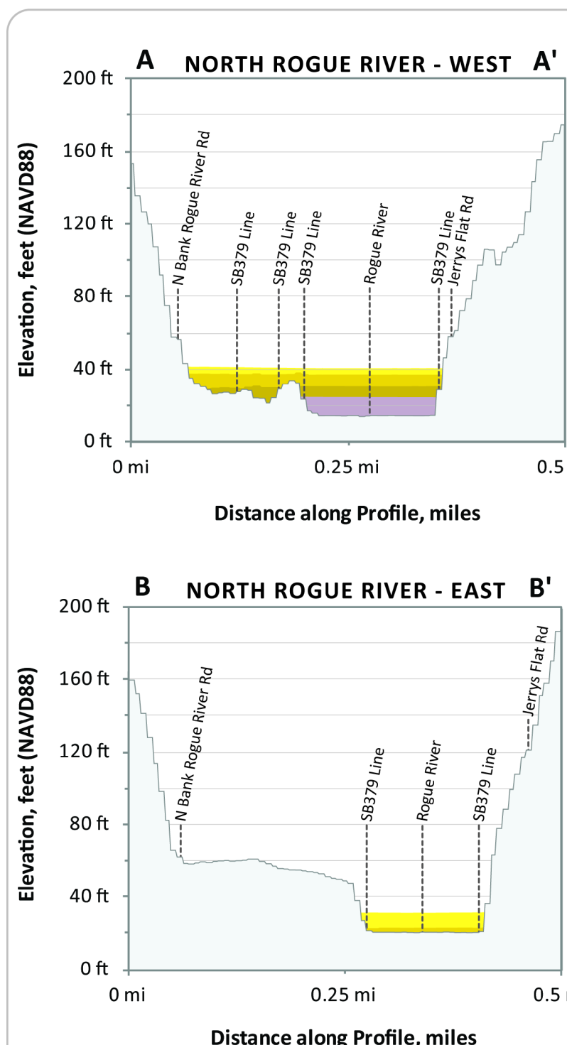
Figure 6: These profiles depict the expected maximum tsunami wave elevation for the five "T-shirt scenarios" along lines A-A' and B-B'. The tsunami scenarios are modeled to occur at a high tide and to account for local subsidence or uplift of the ground surface.
