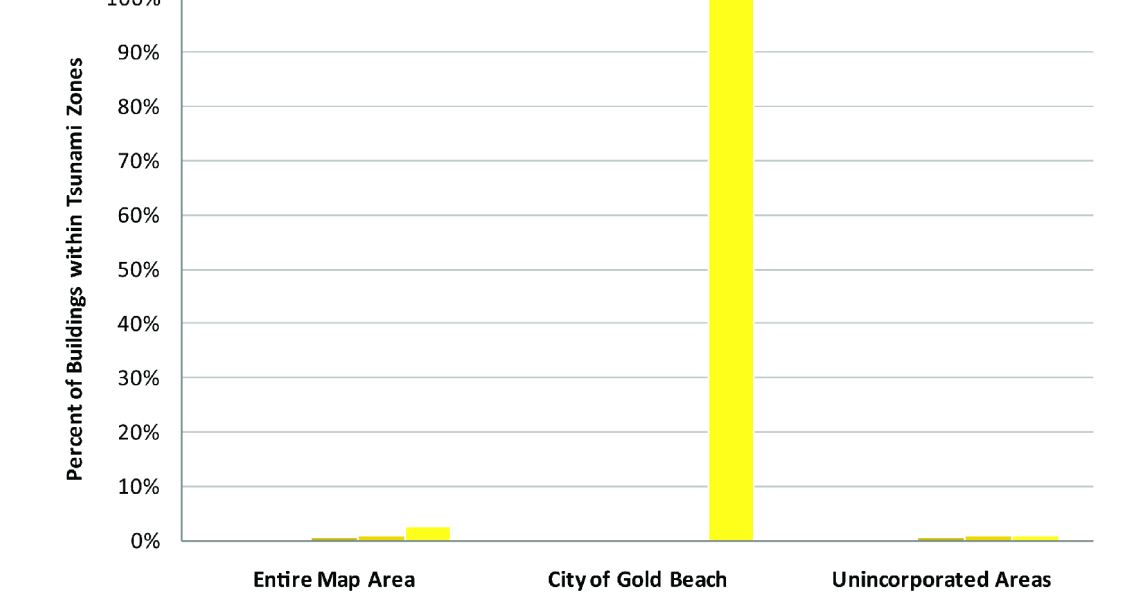
Figure 4: The table and charts show the number of buildings inundated for each "tsunami T-shirt scenario" for cities and unincorporated portions of the map.
