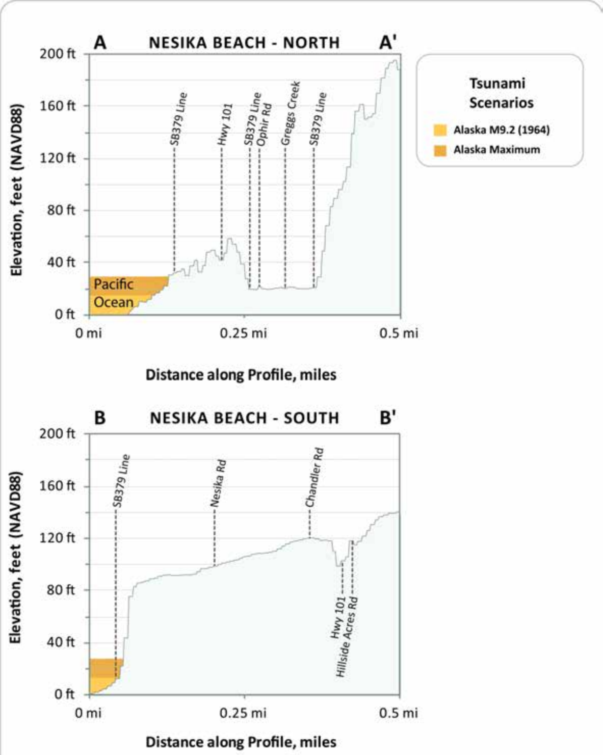
Figure 5. These profiles depict the expected maximum tsunami wave elevation for the two Alaska tsunami scenarios along lines A-A' and B-B'. The tsunami scenarios are modeled to occur at a static (no flow) tide and equal to the Mean Higher High Water (MHHW) high tide.
