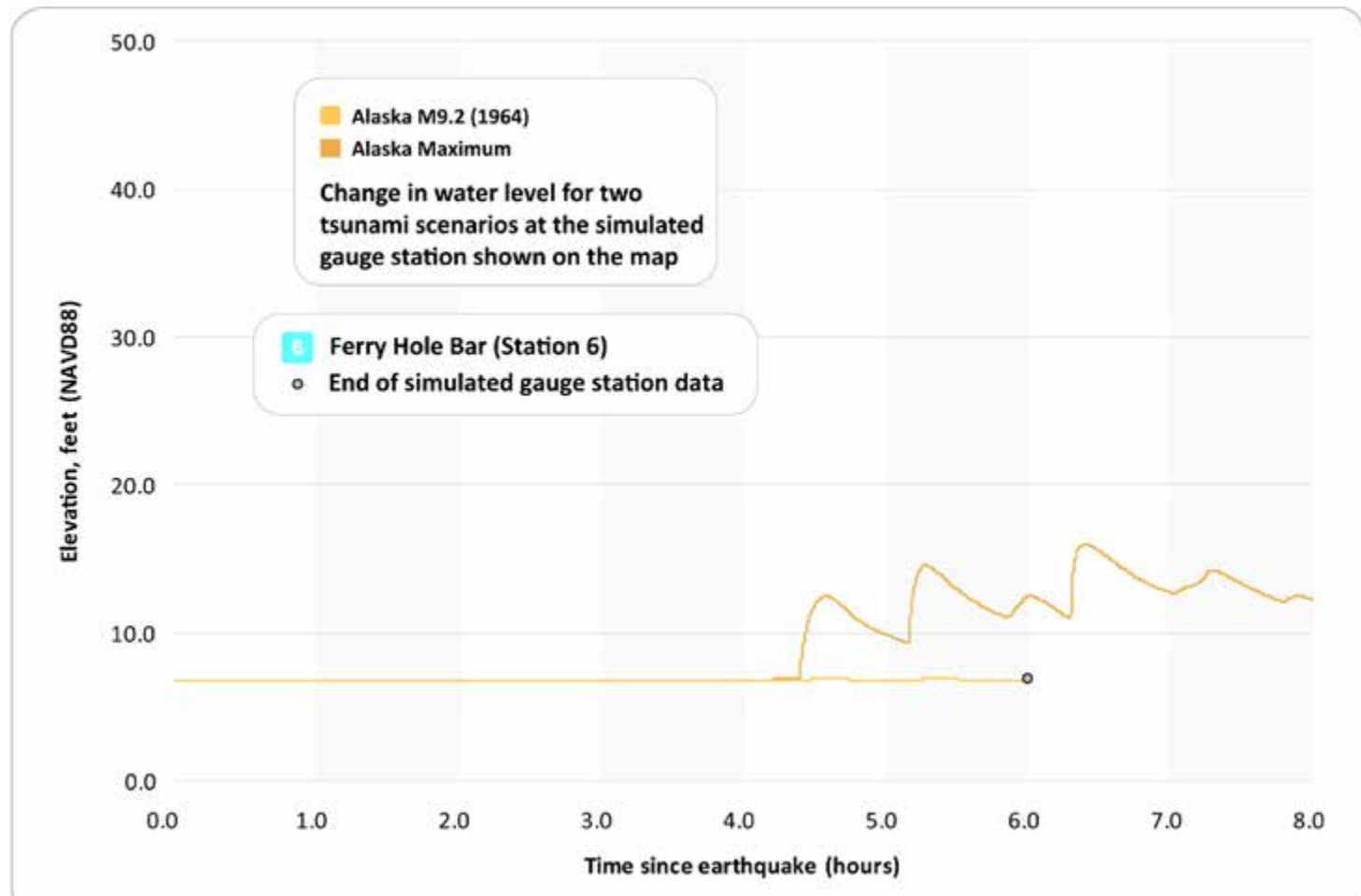
Figure 4. This chart depicts the tsunami waves as they arrive at the selected reference point (simulated gauge station). It shows the change in wave heights for two tsunami scenarios per hour. Wave heights vary through time, and the first wave will not necessarily be the largest as waves interfere and reflect off local topography and bathymetry.
