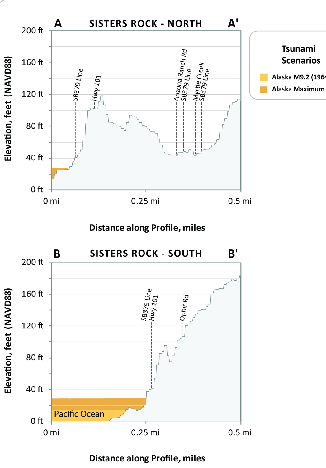
Figure 5: These profiles depict the expected maximum tsunami wave elevation for the two Alaska tsunami scenarios along lines A-A' and B-B'. The tsunami scenarios are modeled to occur at a static (no flow) tide and equal to the Mean Higher High Water (MHHW) high tide.
