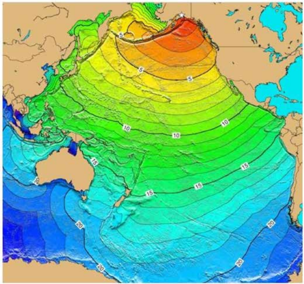
Figure 2. This image depicts the actual initial tsunami arrival time, in hours, around the Pacific rim from the 1964 Prince William Sound earthquake. This magnitude 9.2 earthquake and resulting tsunami caused 125 deaths and $52.1 million in property loss, $84 million and 106 deaths in Alaska (NOAA, 2000). The tsunami devastated many towns along the Gulf of Alaska, left serious damage in British Columbia, Hawaii, and along the west coast of the United States, and was recorded on tide gauges in Cuba and Puerto Rico.
