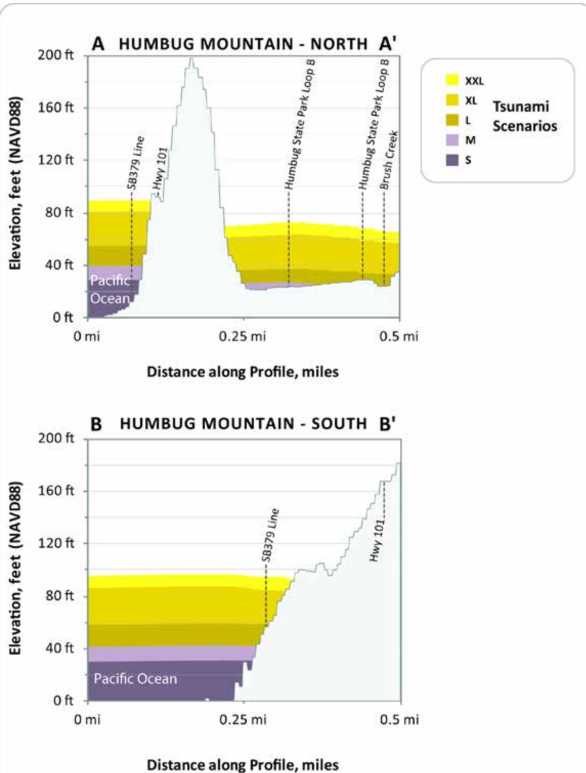
Figure 6: These profiles depict the expected maximum tsunami wave elevation for the five 'tsunami T-shirt scenarios' along lines A-A' and B-B'. The tsunami scenarios are modeled to occur at high tide and to account for local subsidence or uplift of the ground surface.
