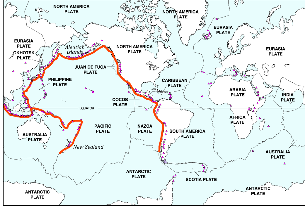
Figure 1: The "Ring of Fire" is a zone of active earthquake and volcano that rings much of the Pacific Ocean, including the Oregon coast. Volcanoes and earthquakes on this ring are caused by the movements of tectonic plates. One type of movement is called subduction – where thin, oceanic plates, such as those that compose the rock beneath the Pacific Ocean, move beneath thicker, lighter plates that make up continental plates. Earthquakes that occur as a result of subduction can trigger tsunamis.
