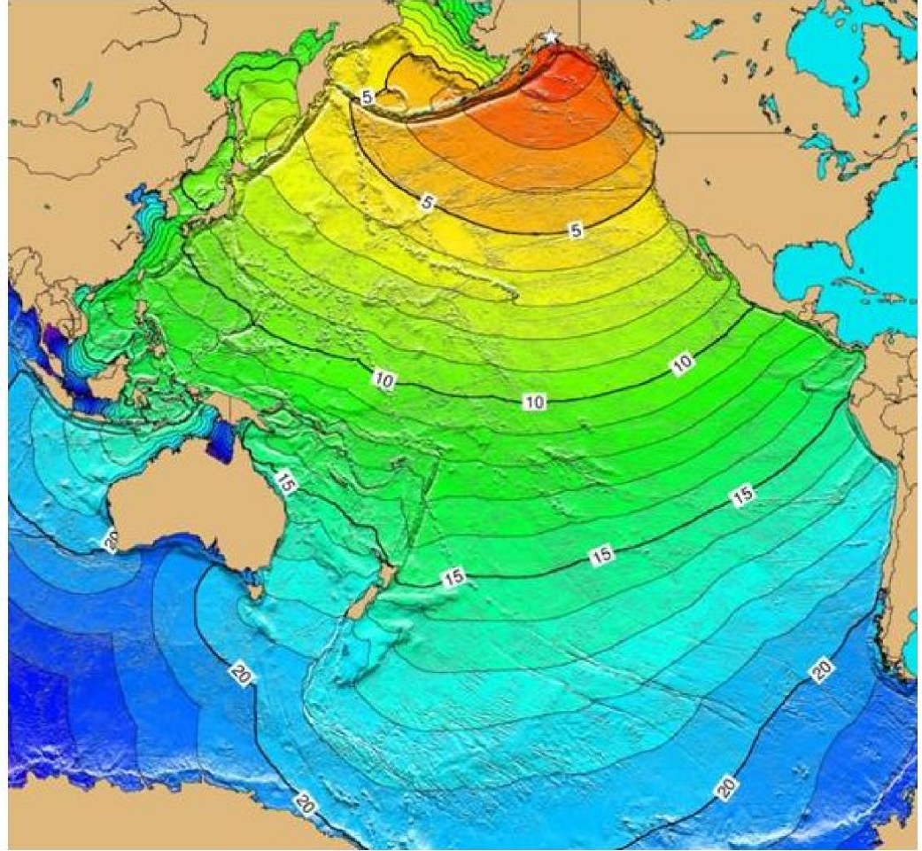
Figure 2: This image depicts the actual initial tsunami arrival times, in hours, around the Pacific Rim from the 1964 Prince William Sound earthquake. This magnitude 9.2 earthquake and resulting tsunami caused 125 deaths and $311 million in property loss, $48 million and 156 deaths in Alaska (NGIC/WDC). The tsunami devastated many towns along the Gulf of Alaska, left serious damage in British Columbia, Hawaii, and along the west coast of the United States, and was recorded on tide gauges in Cuba and Puerto Rico.
