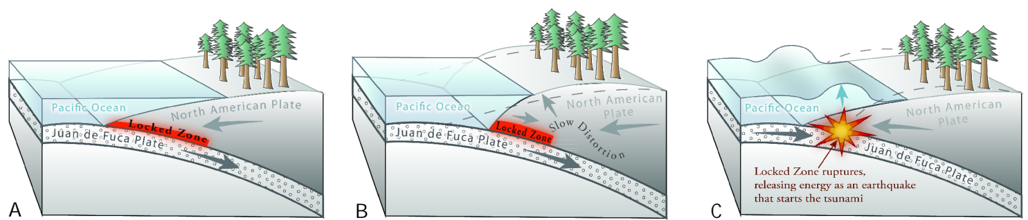
Figure 2: The North American Plate slips over the descending Juan de Fuca Plate at a rate of approximately 1.5 inches per year. Because the two plates are stuck in place at the "locked zone," strain builds up over time and the North American Plate bulges up. Eventually the locked zone ruptures and causes a giant earthquake. The sudden slip of the two plates displaces the Pacific Ocean water upward and creates a tsunami.
