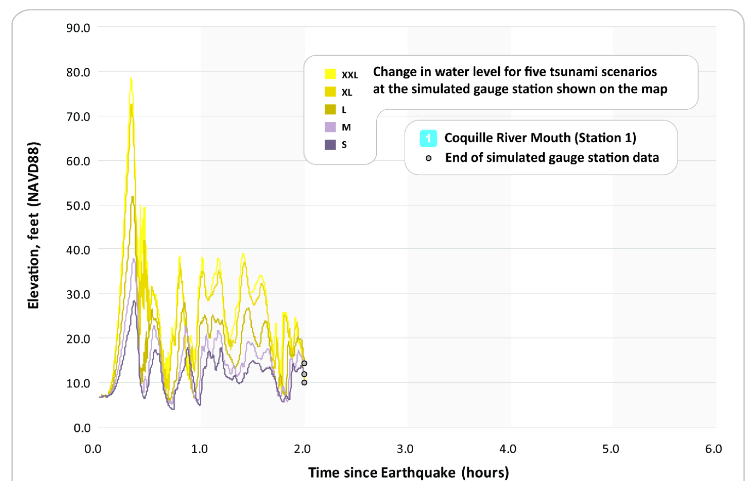
Figure 5: This chart depicts the tsunami waves as they arrive at the selected reference point (simulated gauge station). It shows the change in wave heights for all five tsunami scenarios over an 6-hour period. The starting water elevation (0.0 hour) takes into account the local land subsidence or uplift caused by the earthquake. Wave heights vary through time, and the first wave will not necessarily be the largest as waves interfere and reflect off local topography and bathymetry.
