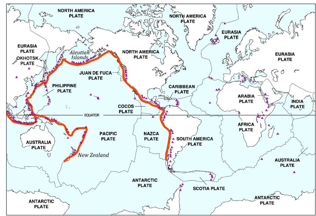
Figure 1: The 'Ring of Fire' is a zone of active earthquakes and volcanoes that ring much of the Pacific Ocean, including the Oregon coast. Volcanoes, and earthquakes on this ring are caused by the movement of tectonic plates. One type of movement is called subduction — when thin, oceanic plates, such as those that compose the rock beneath the Pacific Ocean, sink beneath thicker, lighter plates that make up continental plates. Earthquakes that occur as a result of subduction can trigger tsunamis.
