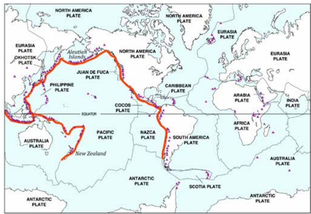
Figure 1: The 'Ring of Fire' is a zone of active earthquakes and volcanoes that ring much of the Pacific Ocean, including the Oregon coast. Volcanoes, and earthquakes on this ring are caused by the movement of tectonic plates. One type of movement is called subduction — when thin, oceanic plates, such as those that compose the rock beneath the Pacific Ocean, sink beneath thicker, lighter plates that make up continental plates. Earthquakes that occur as a result of subduction can trigger tsunamis.
