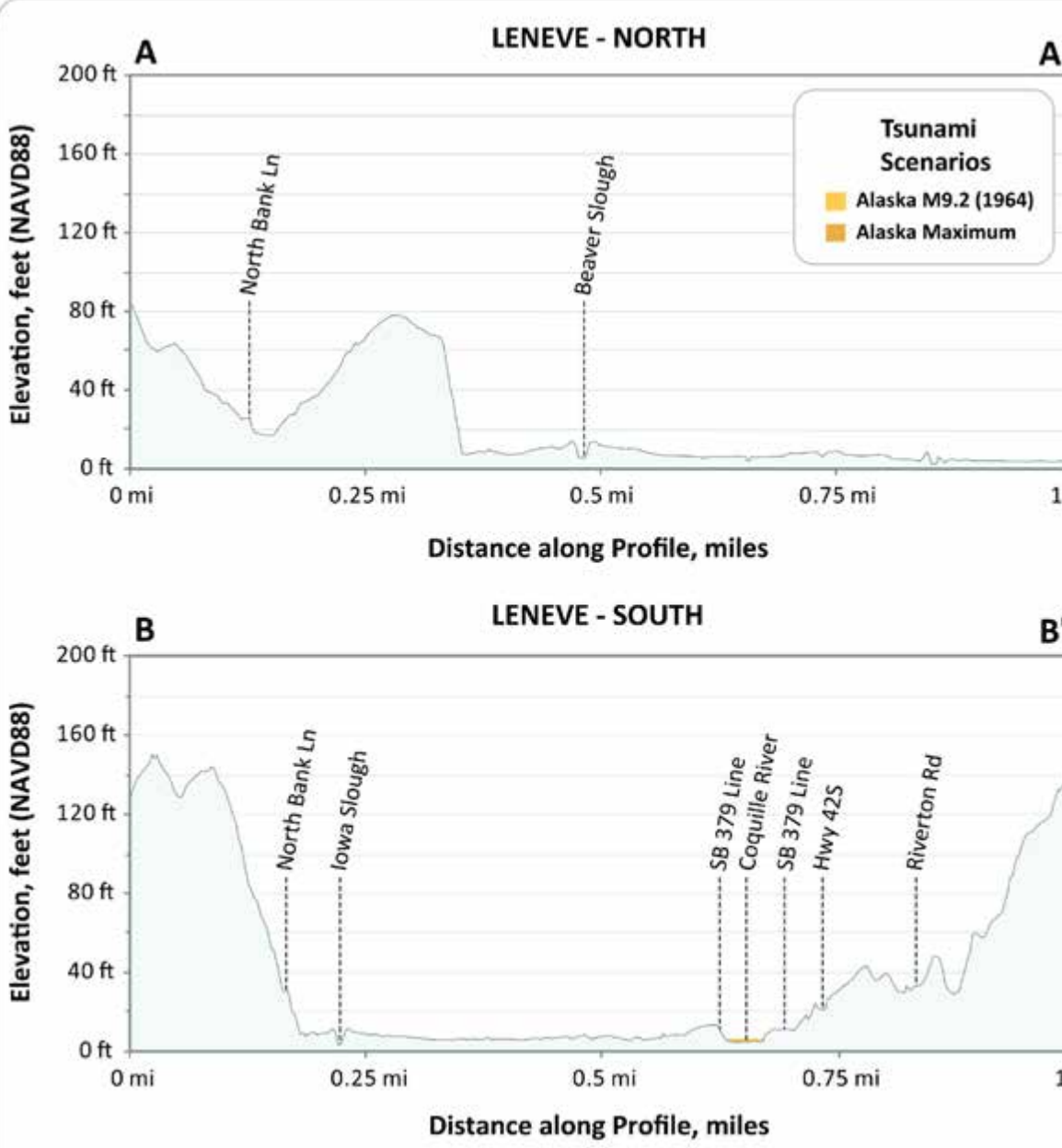
Figure 5: These profiles depict the expected maximum tsunami wave elevation for the two Alaska tsunami scenarios along lines A-A' and B-B'. The tsunami scenarios are modeled to occur at a static (no flow) tide and equal to the Mean Higher High Water (MHHW) high tide.
