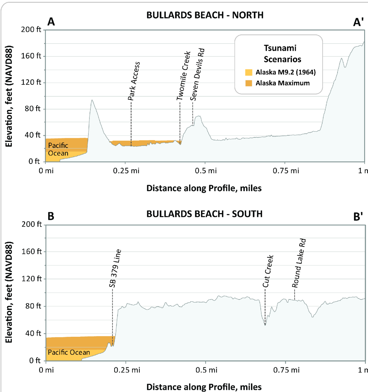
Figure 5: These profiles depict the expected maximum tsunami wave elevation for the two Alaska tsunami scenarios along lines A-A' and B-B'. The tsunami scenarios are modeled to occur at a 'wet' (no flow) tide and equal to the Mean Higher High Water (MHHW) high tide.
