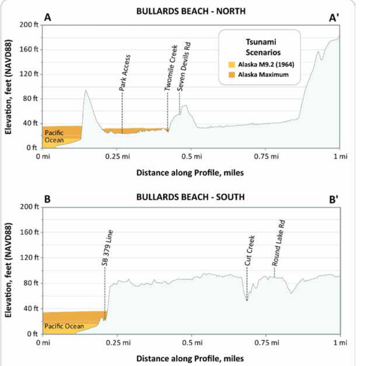
Figure 5: These profiles depict the expected maximum tsunami wave elevation for the two Alaska tsunami scenarios along lines A-A' and B-B'. The tsunami scenarios are modeled to occur at a sea level (on flow) tide and equal to the Mean Higher High Water (MHHW) high tide.
