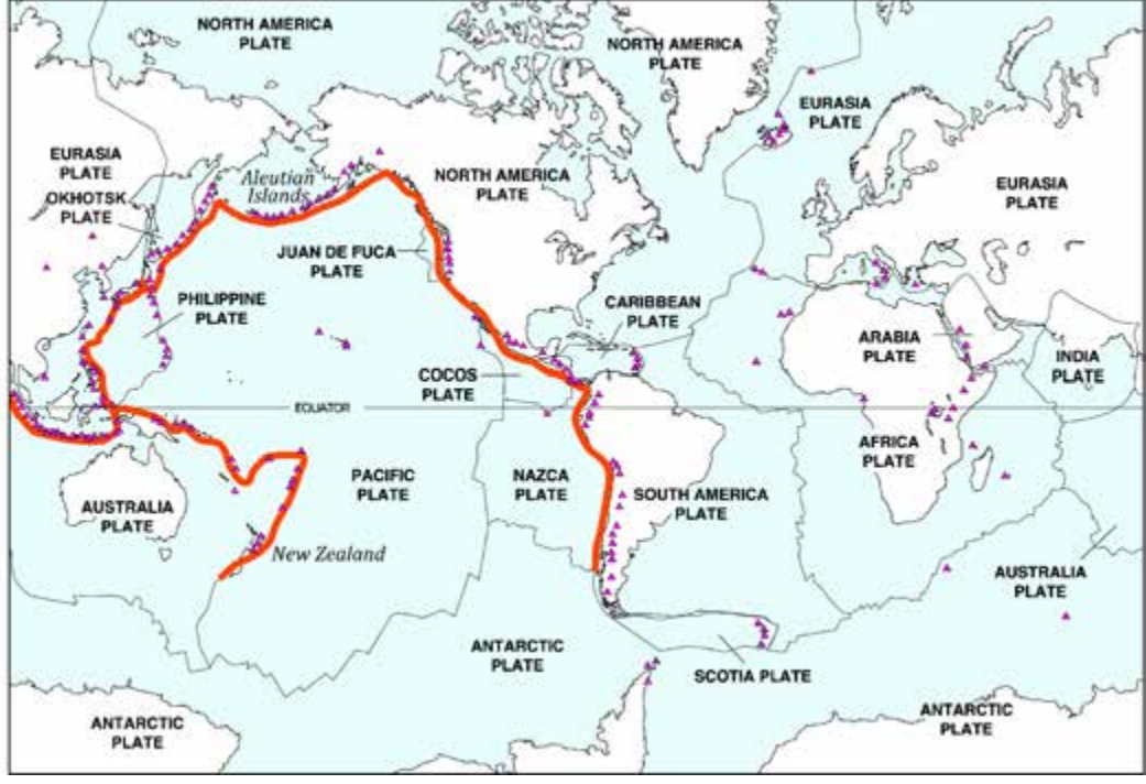
Figure 3: The "Ring of Fire" is a zone of active earthquakes and volcanoes that ring much of the Pacific Ocean, including the Oregon coast. Volcanoes and earthquakes on this ring are caused by the movements of tectonic plates. One type of movement is called subduction – when thin, oceanic plates, such as those that comprise the rock beneath the Pacific Ocean, sink beneath thicker, lighter plates that make up continental plates. Earthquakes that occur as a result of subduction can trigger tsunamis.
