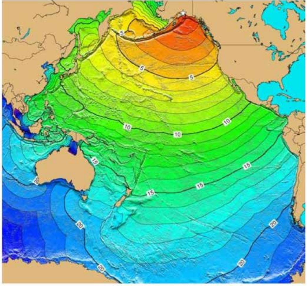
Figure 2: This image depicts the actual initial tsunami arrival time, in hours, around the Pacific from the 1964 Prince William Sound earthquake. This magnitude 9.2 earthquake and resulting tsunami caused 128 deaths and $31 million in property loss, 84 million and 148 deaths in Alaska (NGC-WGC). The tsunami devastated many towns along the Gulf of Alaska, left serious damage in British Columbia, Hawaii, and along the west coast of the United States, and was recorded on tide gauges in Cuba and Puerto Rico.
