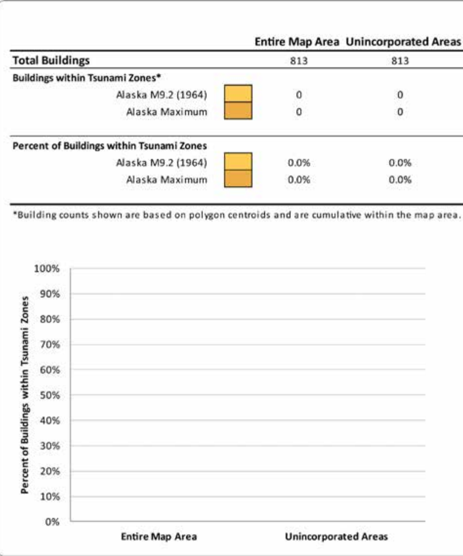
Figure 3: The table and chart show the number of buildings inundated for the Alaska M9.2 (1964) and the Alaska Maximum tsunami scenarios for cities and unincorporated portions of the map.
