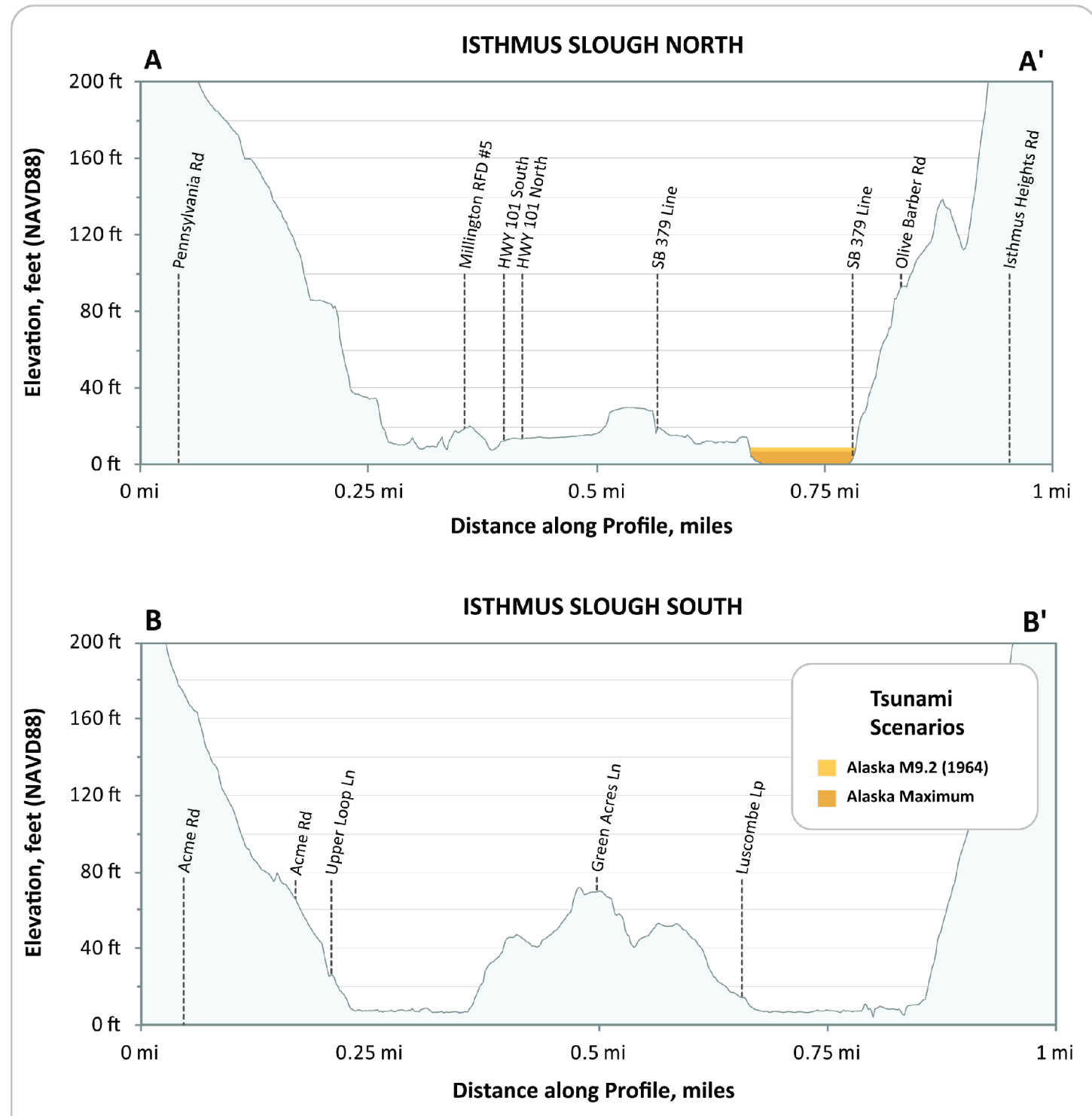
Figure 5: These profiles depict the expected maximum tsunami wave elevation for the two Alaska tsunami scenarios along lines A-A' and B-B'. The tsunami scenarios are modeled to occur at a (a) low (no tide) and equal to the Mean Higher High Water (MHHW) high tide.
