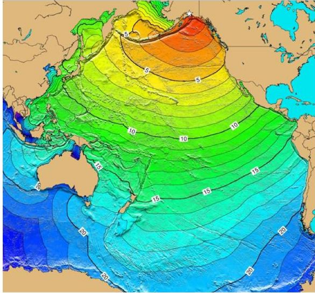
Figure 2: This image depicts the actual initial tsunami travel times in hours, around the Pacific Rim from the 1964 Prince William Sound earthquake. This magnitude 9.2 earthquake and resulting tsunami caused 125 deaths and $311 million in property loss. Six million and 346 deaths in Alaska (NCEM, 2002). The tsunami devastated many towns along the Gulf of Alaska, left serious damage in British Columbia, Hawaii, and along the west coast of the United States, and was recorded on tide gauges in Cuba and Puerto Rico.
