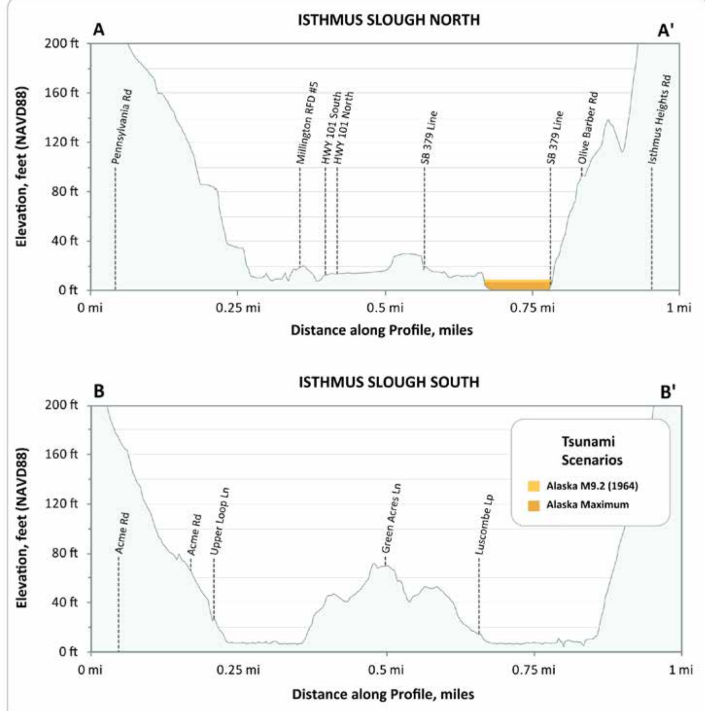
Figure 5. These profiles depict the expected maximum tsunami wave elevation for the two Alaska tsunami scenarios along lines A-A' and B-B'. The tsunami scenarios are modeled to occur at (a) low (no flow) tide and equal to the Mean Higher High Water (MHHW) high tide.
