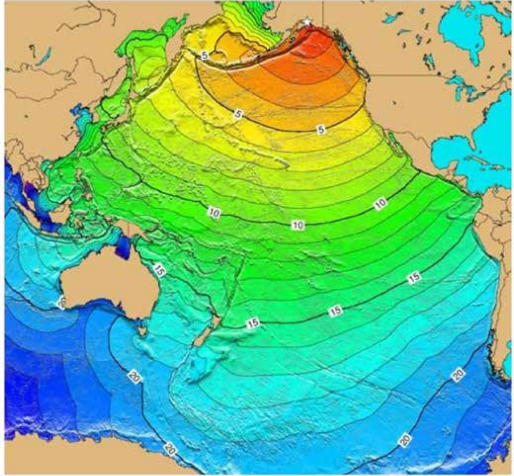
Figure 2. This image depicts the actual initial tsunami arrival times in hours, around the Pacific Rim from the 1964 Prince William Sound earthquake. This magnitude 9.2 earthquake and resulting tsunami caused 125 deaths and $311 million in property loss. 84 million and 136 deaths in Alaska (NGSC-WFO). The tsunami devastated many towns along the Gulf of Alaska, left serious damage in British Columbia, Hawaii, and along the west coast of the United States, and was recorded on tide gauges in Cuba and Puerto Rico.
