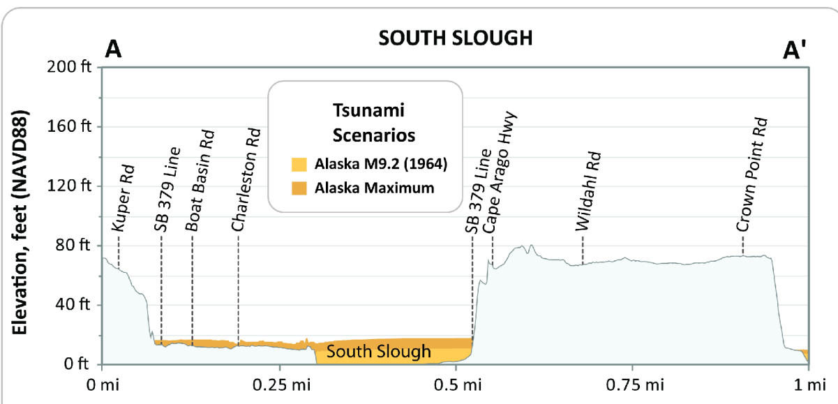
Figure 5: This profile depicts the expected maximum tsunami wave elevation for the two Alaska tsunami scenarios along line A-A'. The tsunami scenarios are modeled to occur at a static (no flow) tide and equal to the Mean Higher High Water (MHHW) high tide.
