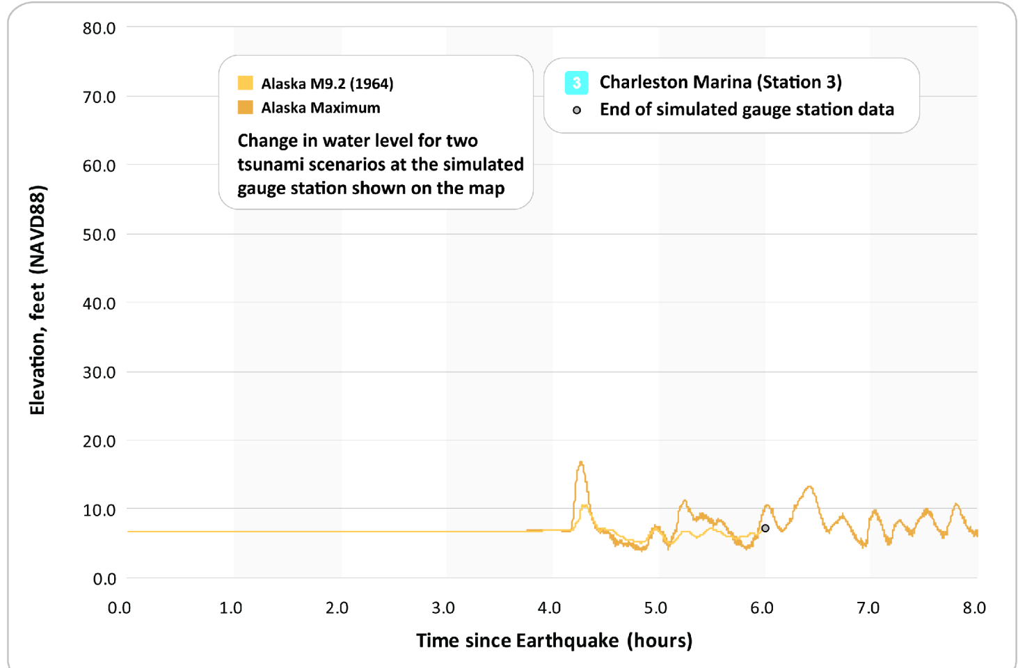
Figure 4: This chart depicts the tsunami waves they arrive at the selected reference point (simulated gauge station). It shows the change in wave heights for the two Alaska tsunami scenarios over an 8-hour period. Wave heights vary through time, and the first wave will not necessarily be the largest as waves can reflect and interact off local topography and bathymetry.
