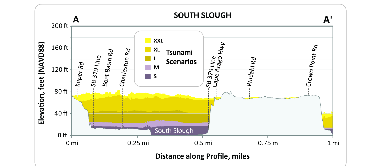
Figure 6: This profile depicts the expected maximum tsunami wave elevation for the five "T-shirt" scenarios along line A-A'. The tsunami scenarios are modeled to occur at high tide and to account for local subsidence or uplift of the ground surface.
