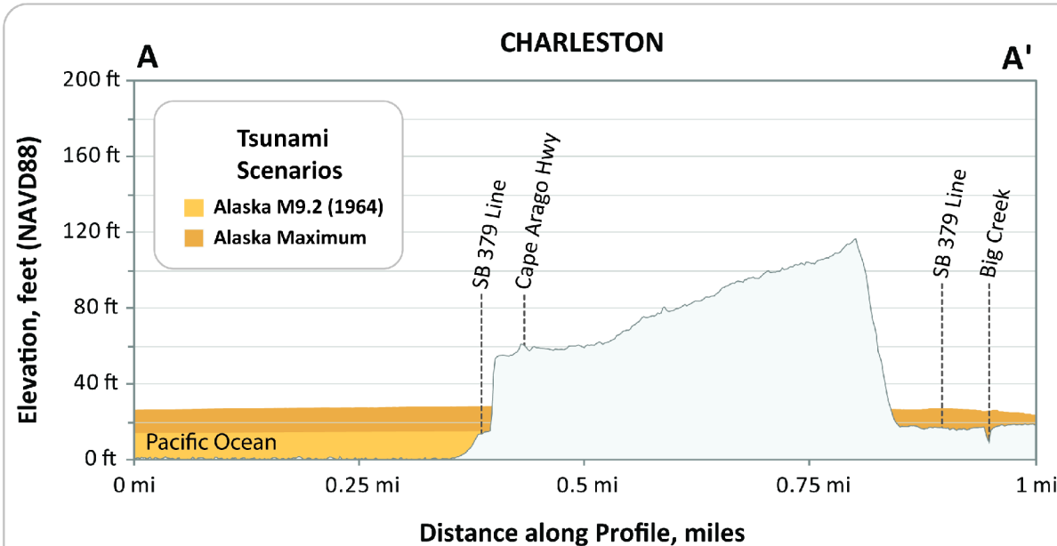
Figure 5: This profile depicts the expected maximum tsunami wave elevation for the two Alaska tsunami scenarios along line A-A. The tsunami scenarios are modeled to occur at a static (fixed) tide and equal to the Mean Higher High Water (MHHW) high tide.
