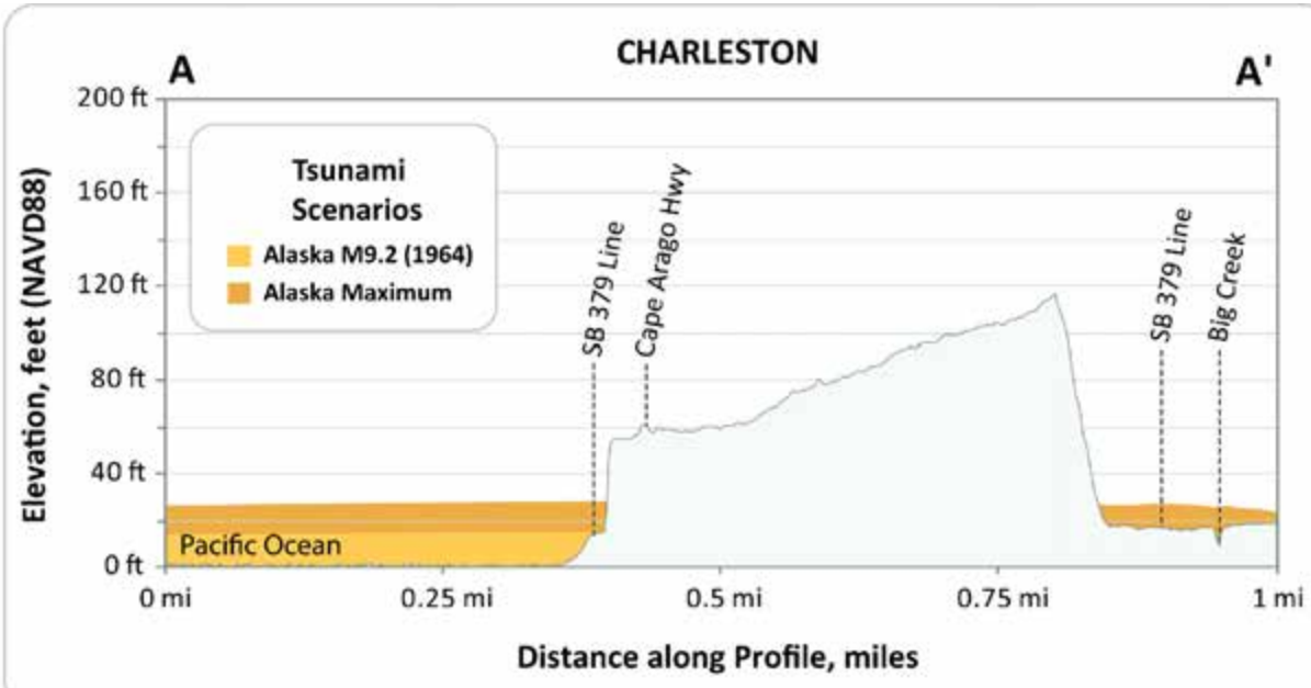
Figure 5: This profile depicts the expected maximum tsunami wave elevation for the two Alaska tsunami scenarios along line A-A. The tsunami scenarios are modeled to occur at a static (no-flow) tide and equal to the higher high water (HHW) high tide.
