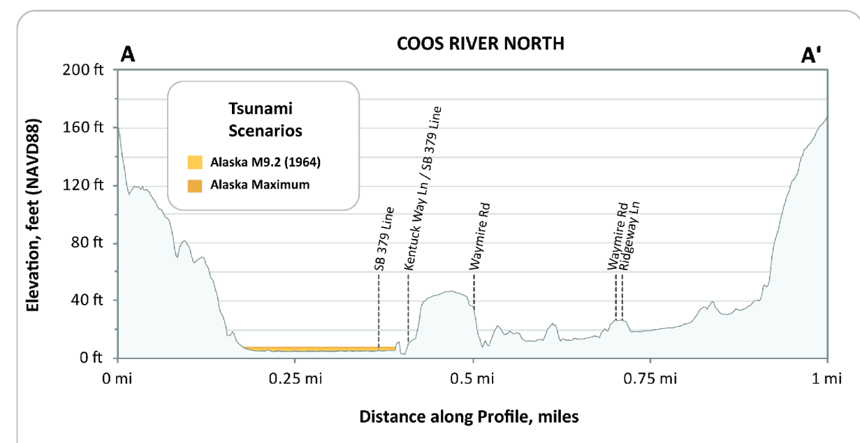
Figure 5: This profile depicts the expected maximum tsunami wave elevation for the two Alaska tsunami scenarios along line A-A'. The tsunami scenarios are modeled to occur at static (no flow) tide and equal to the Mean Higher High Water (MHHW) high tide.
