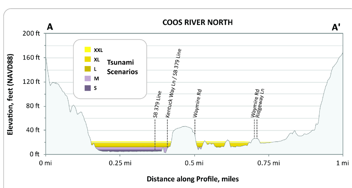
Figure 6. This profile depicts the expected maximum tsunami wave elevation for the five "T-shirt size" scenarios along line A-A'. The tsunami scenarios are modeled to occur at high tide and to account for local subsidence or uplift of the ground surface.
