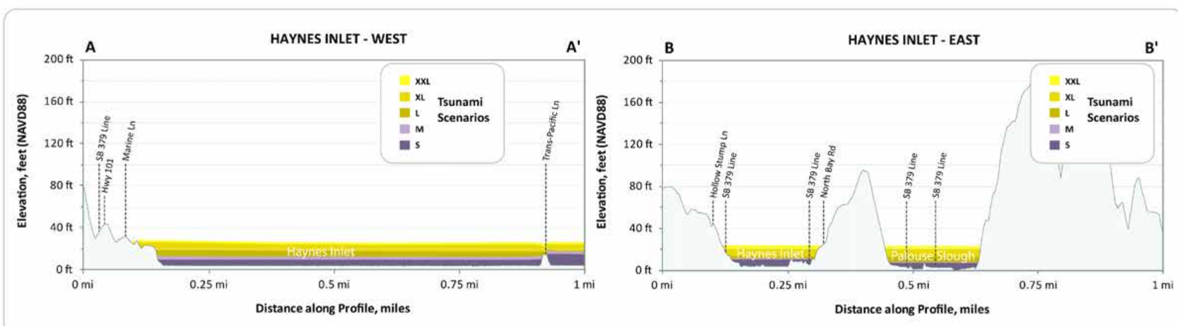
Figure 6. These profiles depict the expected maximum tsunami wave elevation for the five "Tsunami T-shirt scenarios" along lines A-A' and B-B'. The tsunami scenarios are modeled to occur at high tide and to account for local subsidence or uplift of the ground surface.
