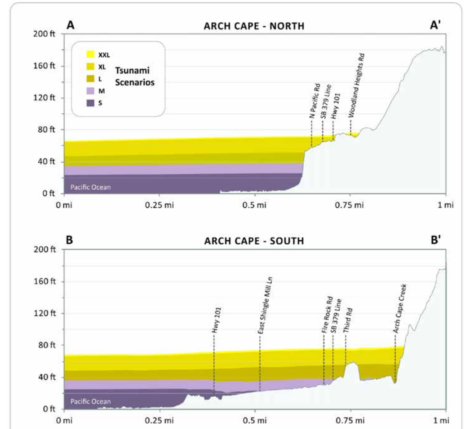
Figure 6. These profiles depict the expected maximum tsunami wave elevation for the five "tsunami T-shirt scenarios" along lines A-A' and B-B'. The tsunami scenarios are modeled to occur at high tide and to account for local subsidence or uplift of the ground surface.
