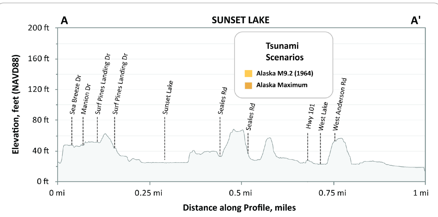
Figure 5: This profile depicts the expected maximum tsunami wave elevation for the two Alaska tsunami scenarios along lines A-A'. The tsunami scenarios are modeled to occur at a static (no flow) tide and equal to the Mean Higher High Water (MHHW) high tide.
