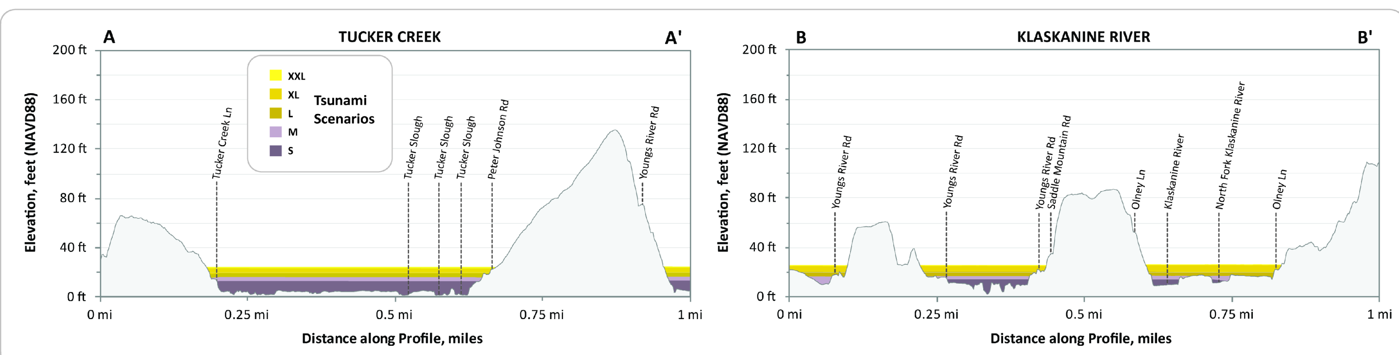
Figure 6: These profiles depict the expected maximum tsunami wave elevation for the five "T-shirt size" scenarios along lines A-A' and B-B'. The tsunami scenarios are modeled to occur at high tide and to account for local subsidence or uplift of the ground surface.
