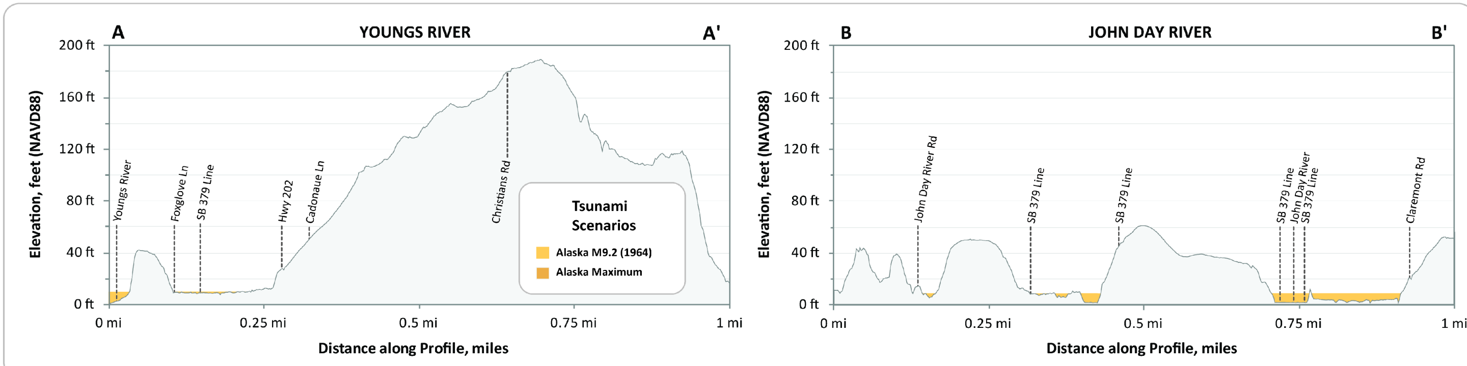
Figure 5: These profiles depict the expected maximum tsunami wave elevation for the two Alaska tsunami scenarios along lines A-A' and B-B'. The tsunami scenarios are modeled to occur at a static (no flow) tide and equal to the Mean Higher High Water (MHHW) high tide.
